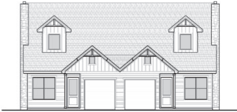
1.5 STORY FRONT ELEVATION
