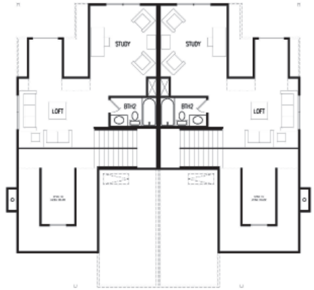
1.5 STORY SECOND FLOOR PLAN
