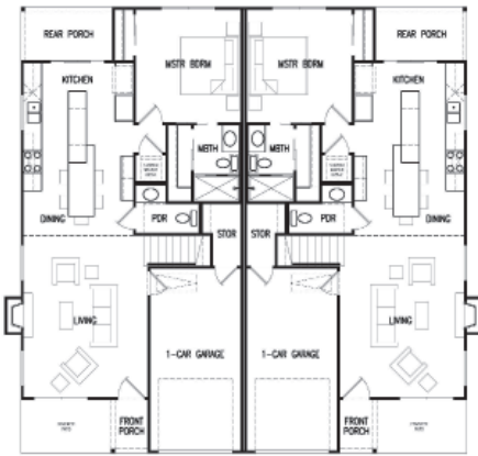
1.5 STORY FIRST FLOOR PLAN
