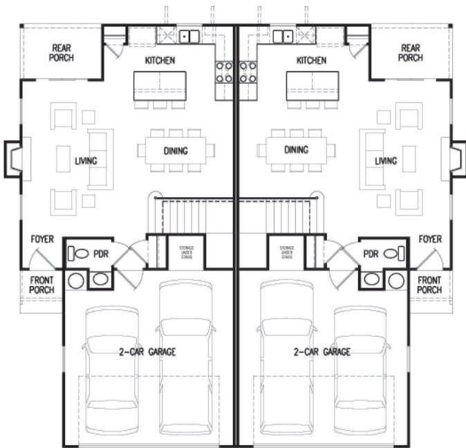
2 STORY FIRST FLOOR PLAN
